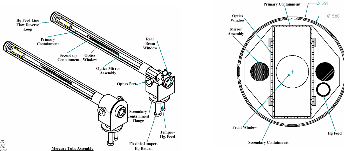
Mercury Tube Assembly
