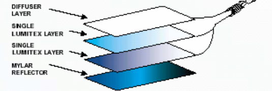
Typical fiber optic panel construction
