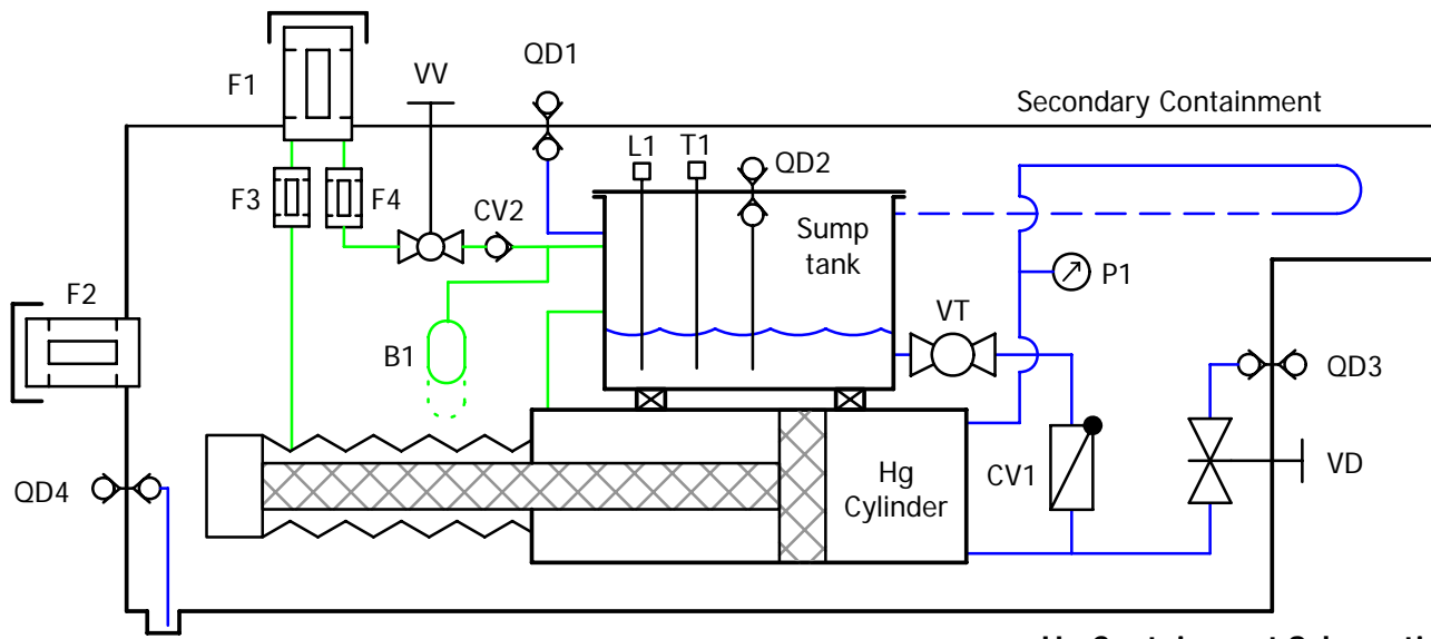
Hg Containment Schematic 8Feb2007
