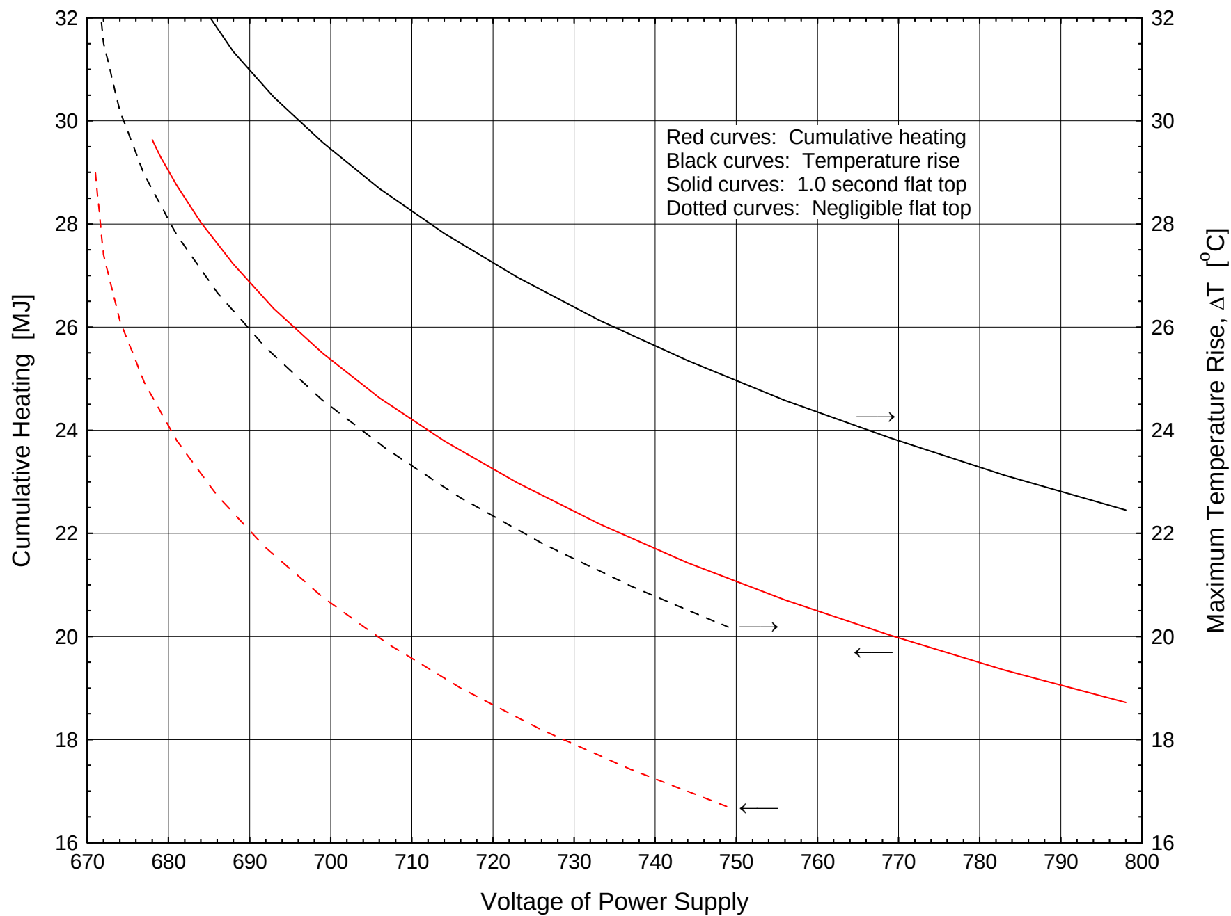
Heating and \Delta T ( T_0 = 82 K) vs. Voltage for E951 Magnets with & without 1 s Flat Top
