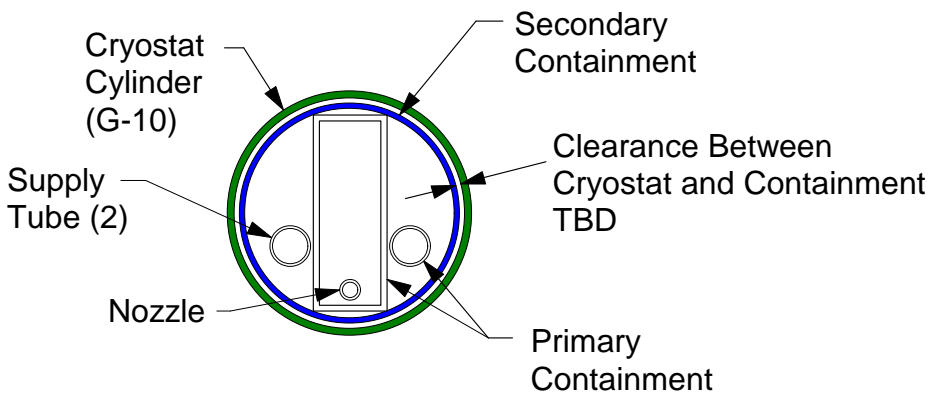
Sect. A-A
