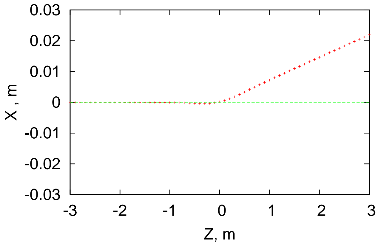
24 GeV Beam - 67 mrad - 15T
